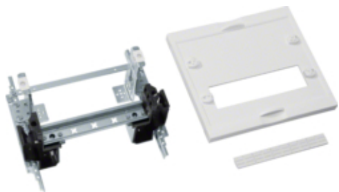
Kit, UniversN, 225x250mm, 1x10module
